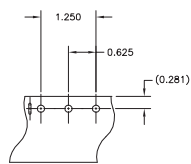
DETAIL A HOLE PATTERN TYP 45 PLACES SCALE 1:1
